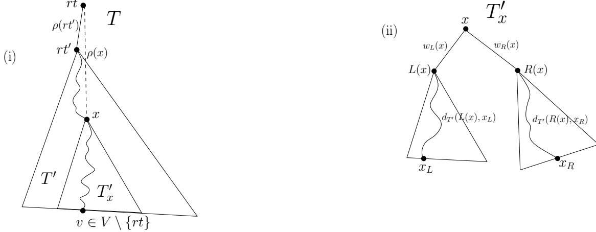
Figure 2. (i) The tree (T, rt) is obtained from T' by adding to it an edge (rt, rt') of weight \rho(rt') . By (1), d_{T'}(x, v) = \text{dist}(rt, v) - \rho(x) . Hence d_T(rt, x) = d_T(rt, v) - d_{T'}(x, v) = (d_T(rt, v) - \text{dist}(rt, v)) + \rho(x) = \rho(x) . The last equation holds because, as we will show in the sequel, T is an SPT with respect to rt . (ii) The path that connects x_L with x_R in T'_x has weight d_{T'}(L(x), x_L) + w_L(x) + w_R(x) + d_{T'}(R(x), x_R) .
